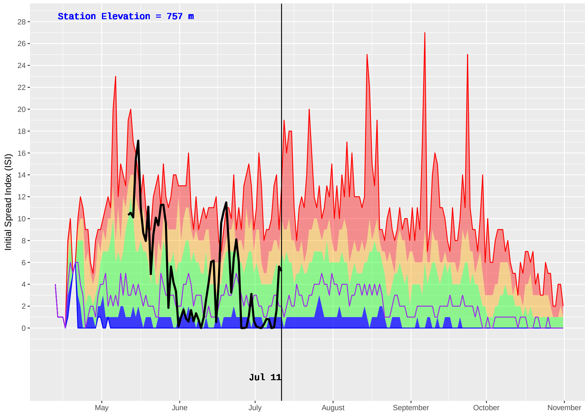
LEMORAY (140) : Historical (1988–2016) and Current (2018) Noon Initial Spread Index (ISI)
