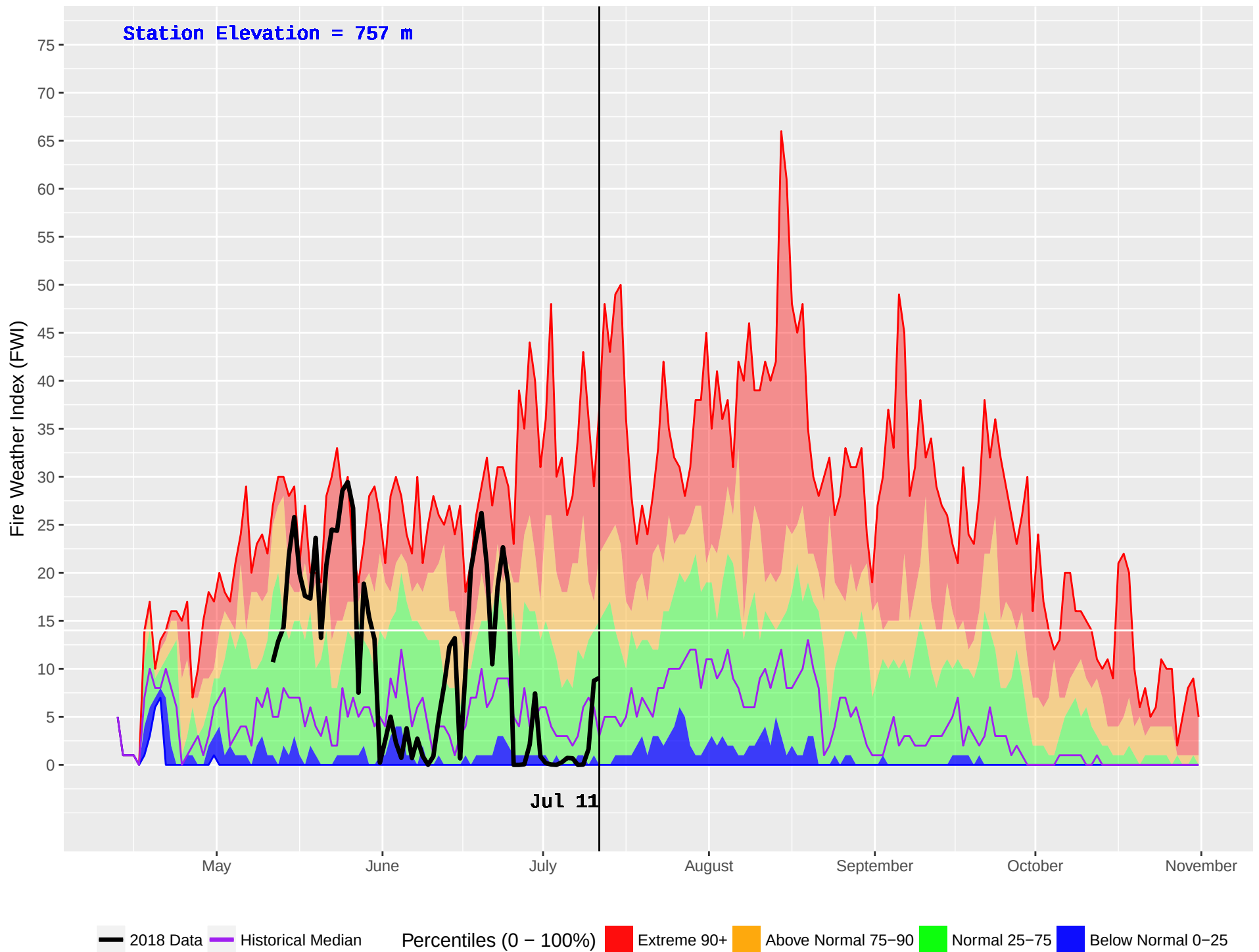
LEMORAY (140) : Historical (1988–2016) and Current (2018) Noon Fire Weather Index (FWI)
